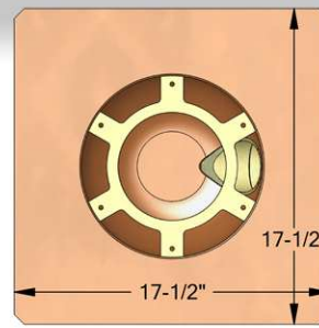
Bottom Outlet Roof Drain ICC-ES PMG-1212
