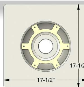
TPO/PVC-Clad Bottom Outlet Roof Drain
