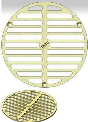
High Volume Round Grate Fits BD6A/F Deck Drain 14.15 in 2 of grate-free area Available in the following finishes: brass (as shown) polished chrome oil-rubbed bronze
