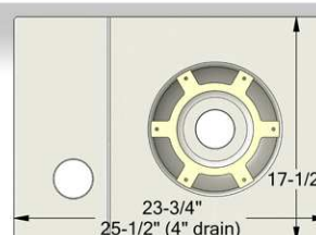
TPO/PVC-Clad Bottom Outlet Roof Drain w/ Overflow
