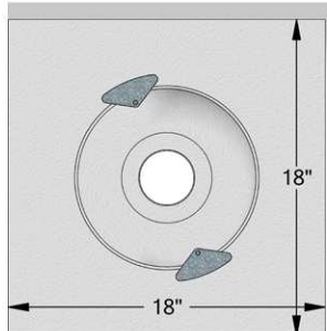
TPO/PVC-Clad Bottom Outlet Roof Drain
