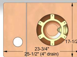
Bottom Outlet Roof Drain w/ Overflow ICC-ES PMG-1212
