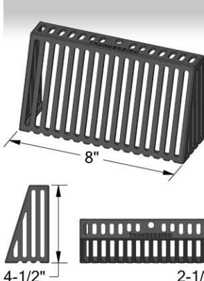
Cast Aluminum Parapet Grate Fits all Thunderbird Parapet Drains A-PDGRATE strainer, black
